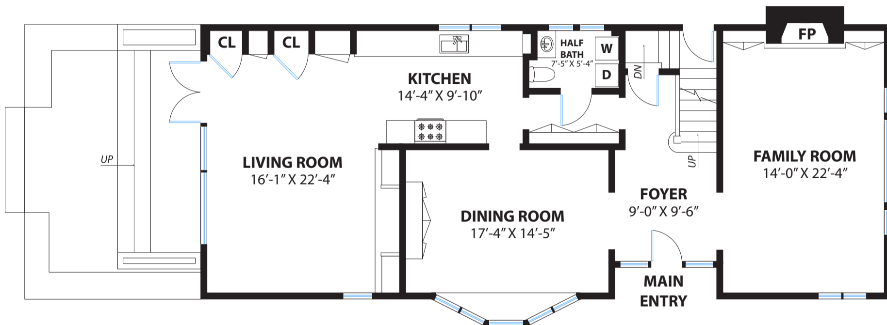
MAIN LEVEL
