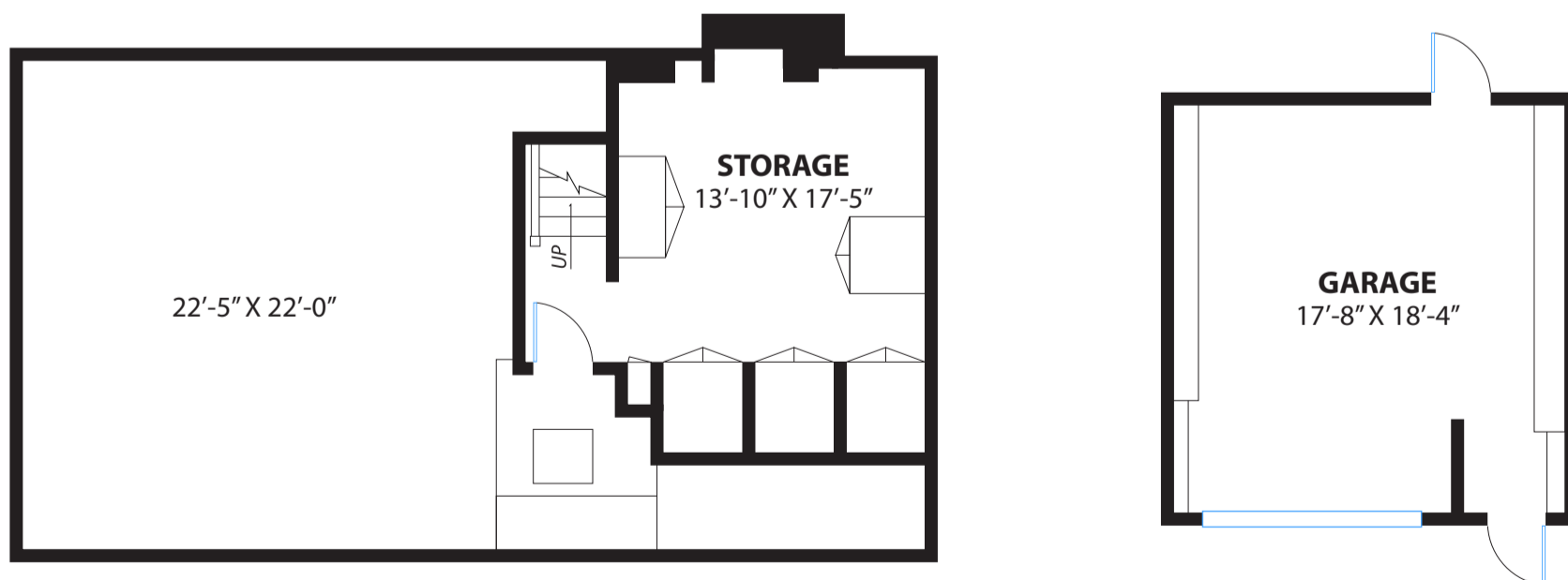
LOWER LEVEL
